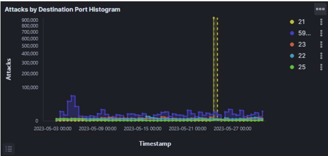
Figure 14: Attacks by Destination Port Histogram
