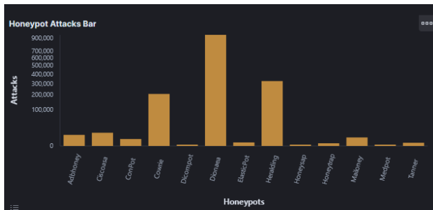
Figure 1 : Honeypots Attacks Bar
