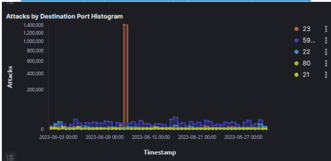
Figure 14: Attacks by Destination Port Histogram
