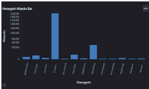
Figure 1 : Honeypots Attacks Bar
