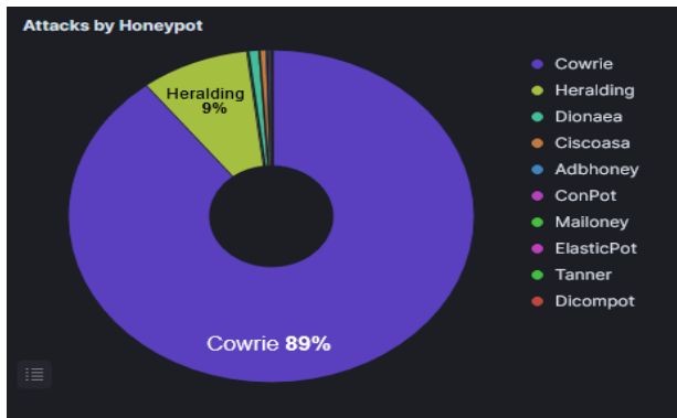
Figure 2: Honeypots Attacks Pie chart
