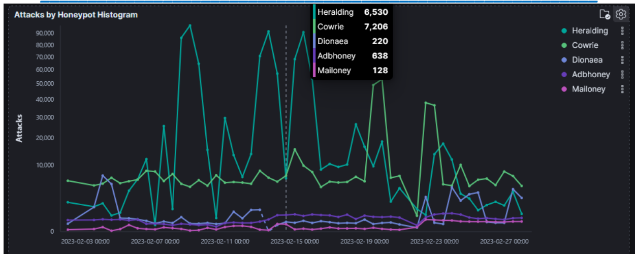
Figure 15: Attacks by Honeypot Histogram
