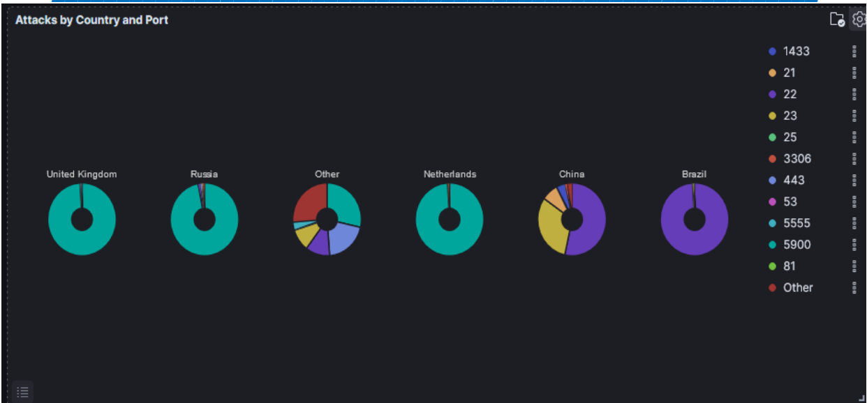
Figure 5 : Attacks by country and port
