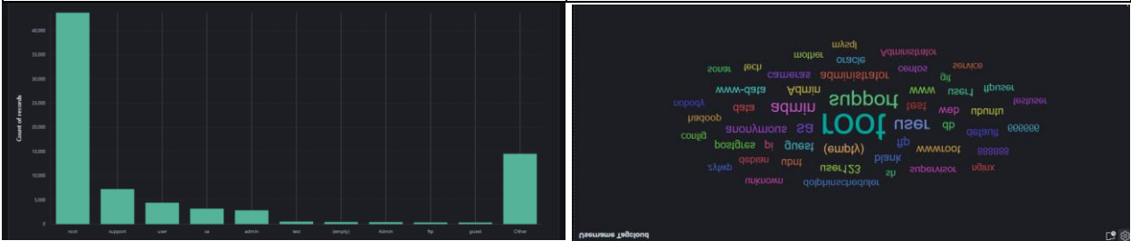
Figure 7: Common usernames used by attackers
